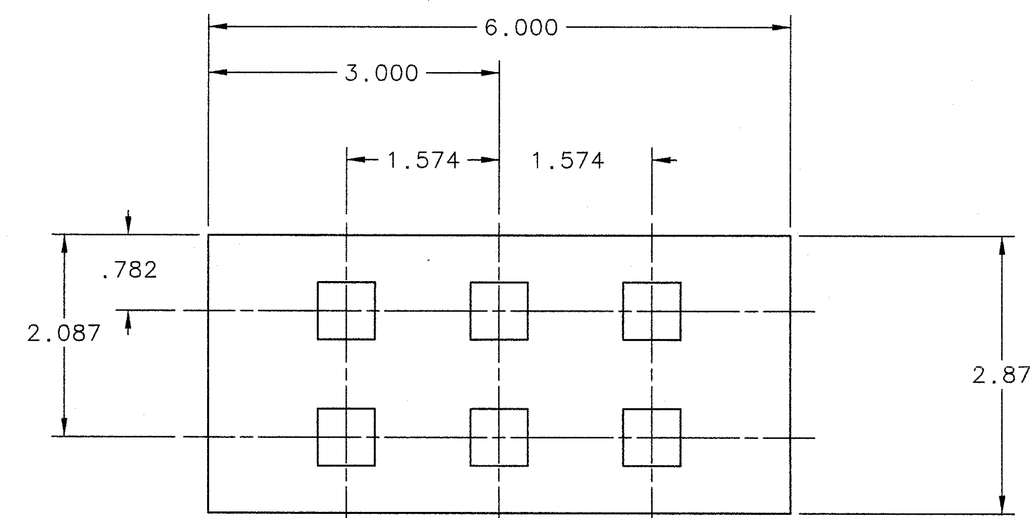
-15 AFT TARGET BRKT 1/1 FOR DETAILS NOT SHOWN, SEE ITEM 14
